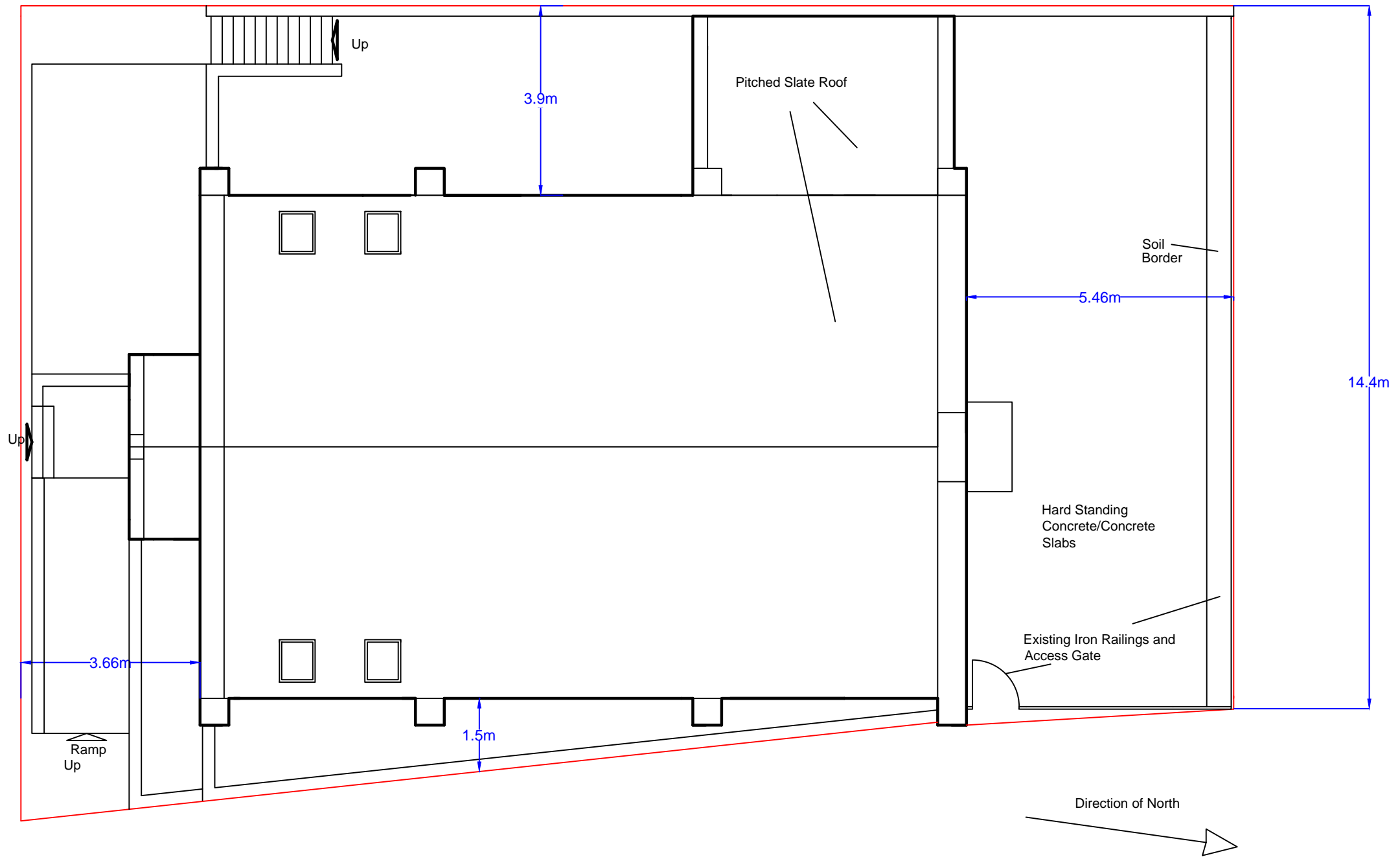
8DT1: 8 Derby Terrace Site Plan As Is Page 1 of 1, Scale 1:100
